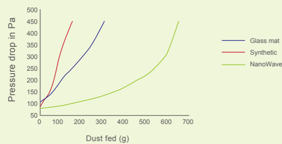
Filter dustloading(g)vs.Pressure drop(Pa)
