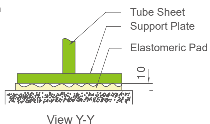
Simplified Isolation
