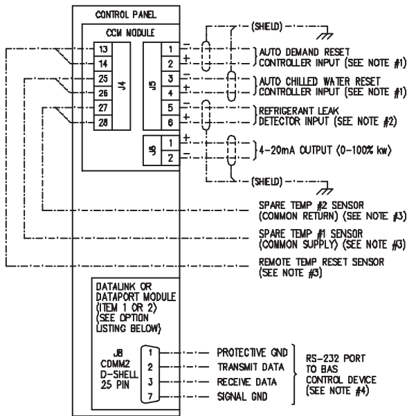
CONTROL PANEL OPTIONAL WIRING
