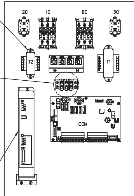
CONTROL PANEL COMPONENT LAYOUT
